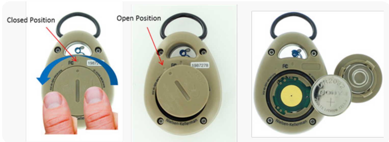
Figure 2: Battery Replacement
