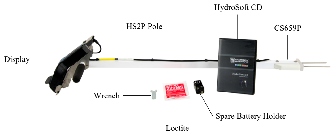
FIGURE 4-3. HS2P Parts
